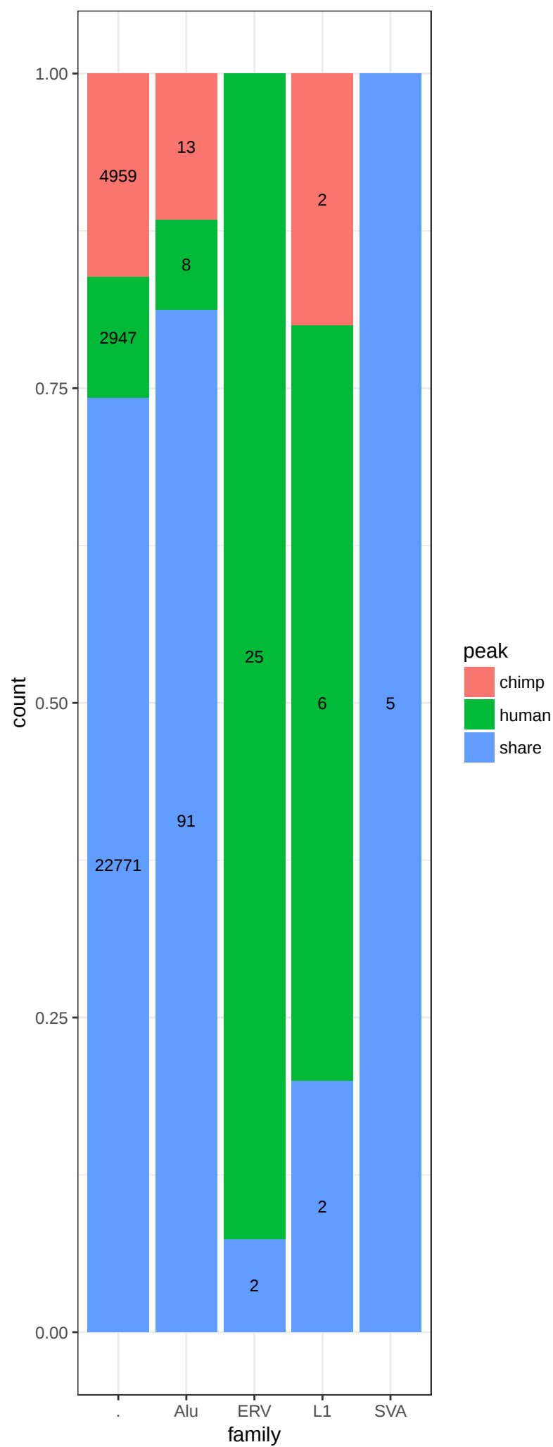
Human iPSC insertion K27ac
