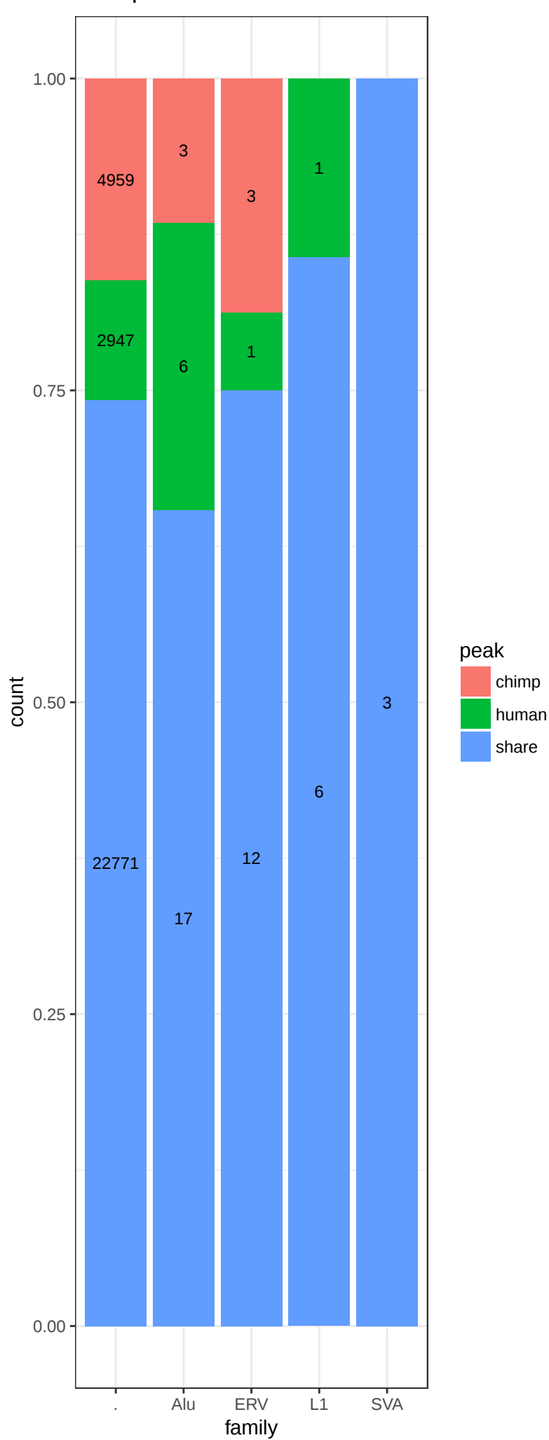
Chimp iPSC insertion K27ac
