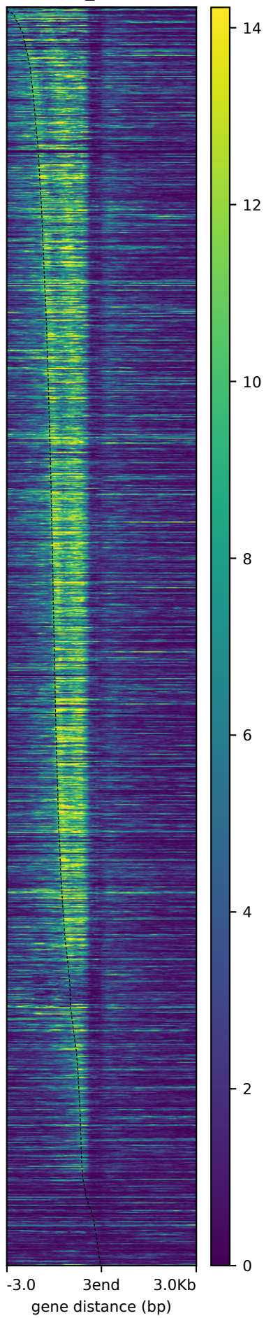
iPSC_K9me3
