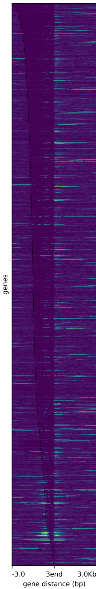
CNCC_K27ac
