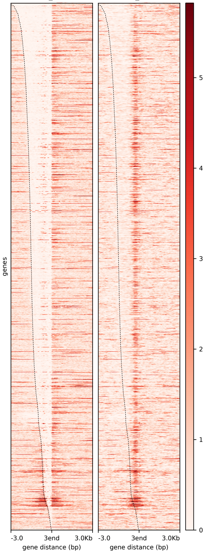
CNCC_K27ac
