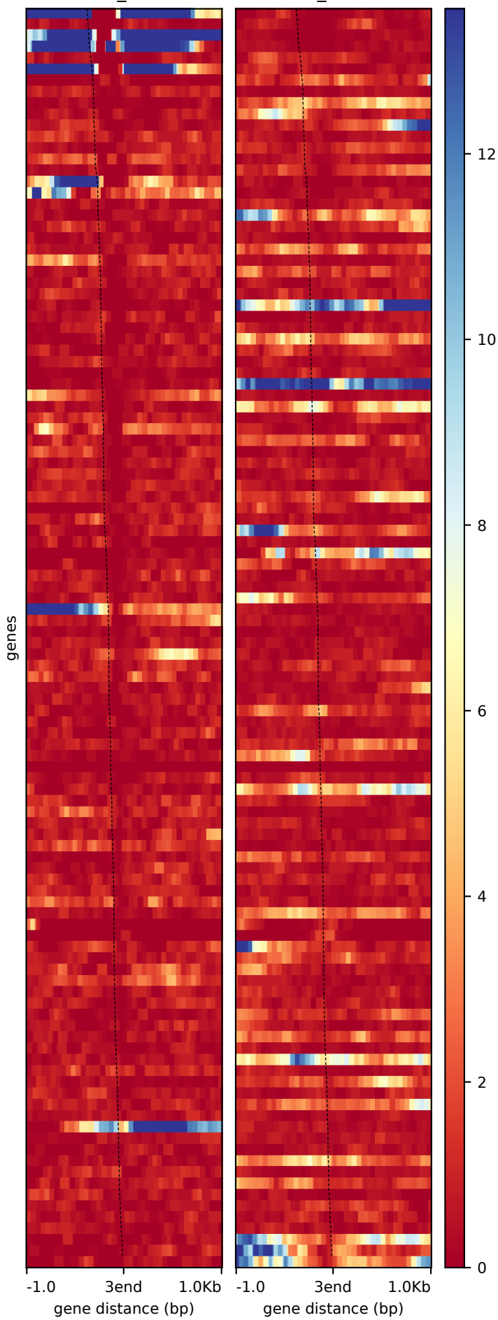
CNCC_K27ac
