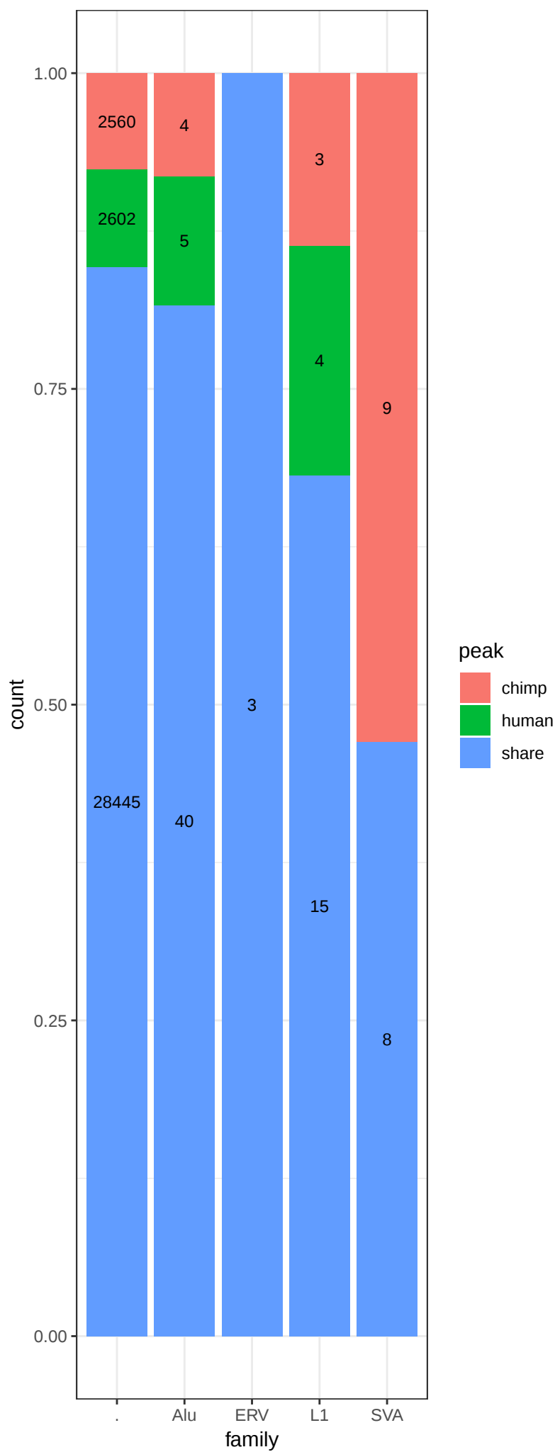
Chimp insertion K27ac
