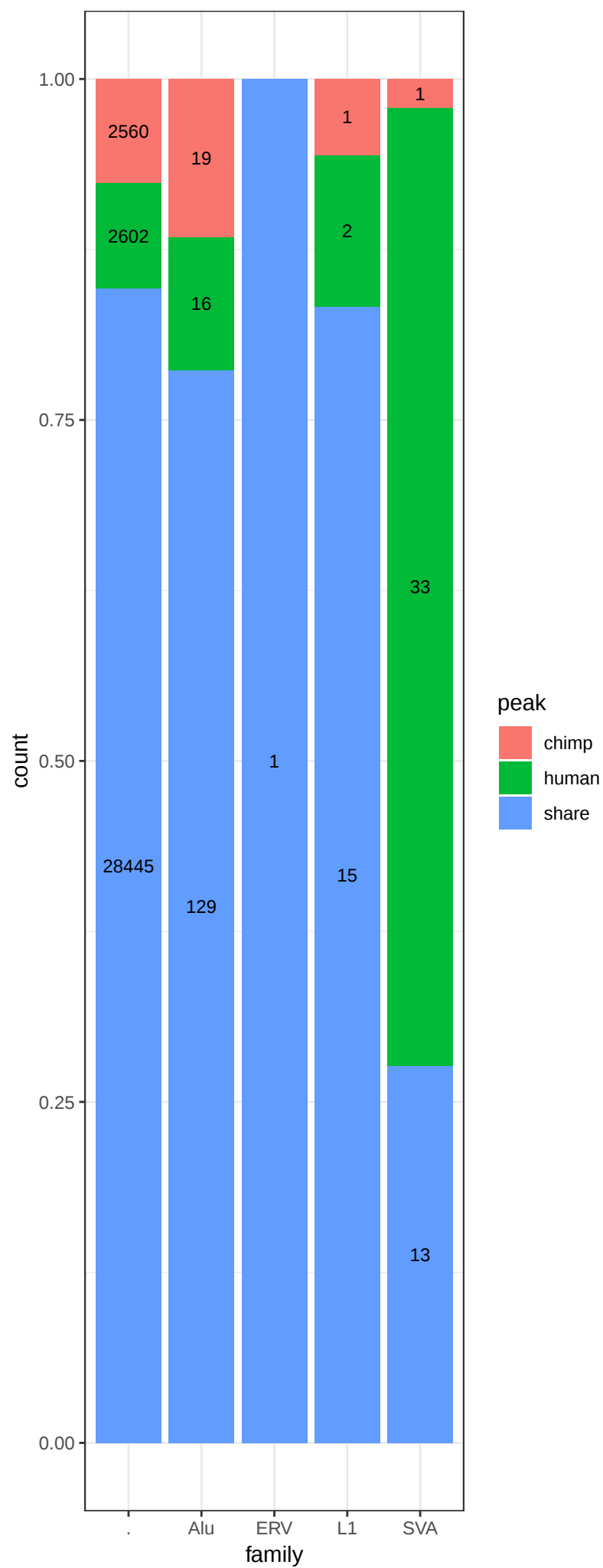
Human insertion K27ac
